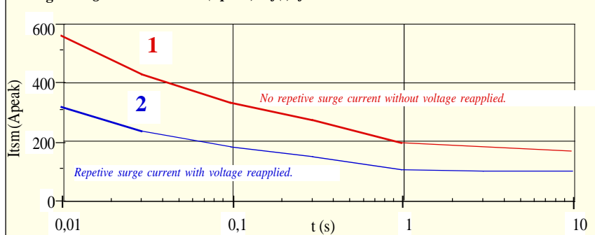
Fig.3 Surge current : I_{tsm} (\text{Apeak}) = f(t) for 50A models with I_{tsm} = 550\text{A}
